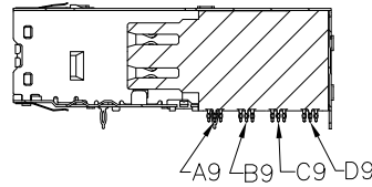
SECTION Z-Z
