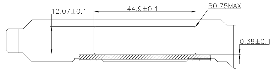
I/O BRACKET CUT OUT (BRACKET NOT SUPPLIED)
