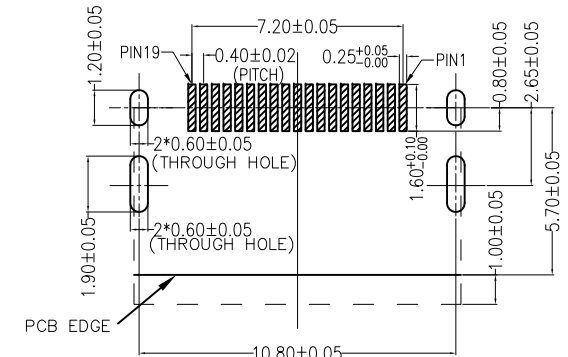
RECOMMENDED PCB LAYOUT(t=0.60±0.10) COMPONENT SIDE
