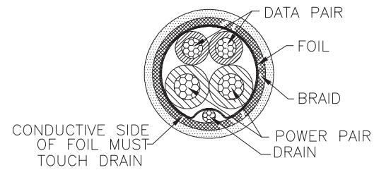
USB CABLE CROSS SECTION SCALE: NONE
